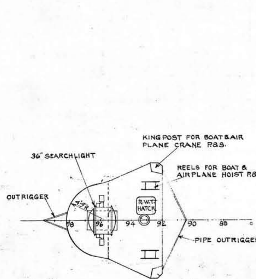
SEARCHLIGHT PLATFORM NO CAMBER NO SHEER 53'-4" ABOVE BASE LINE
